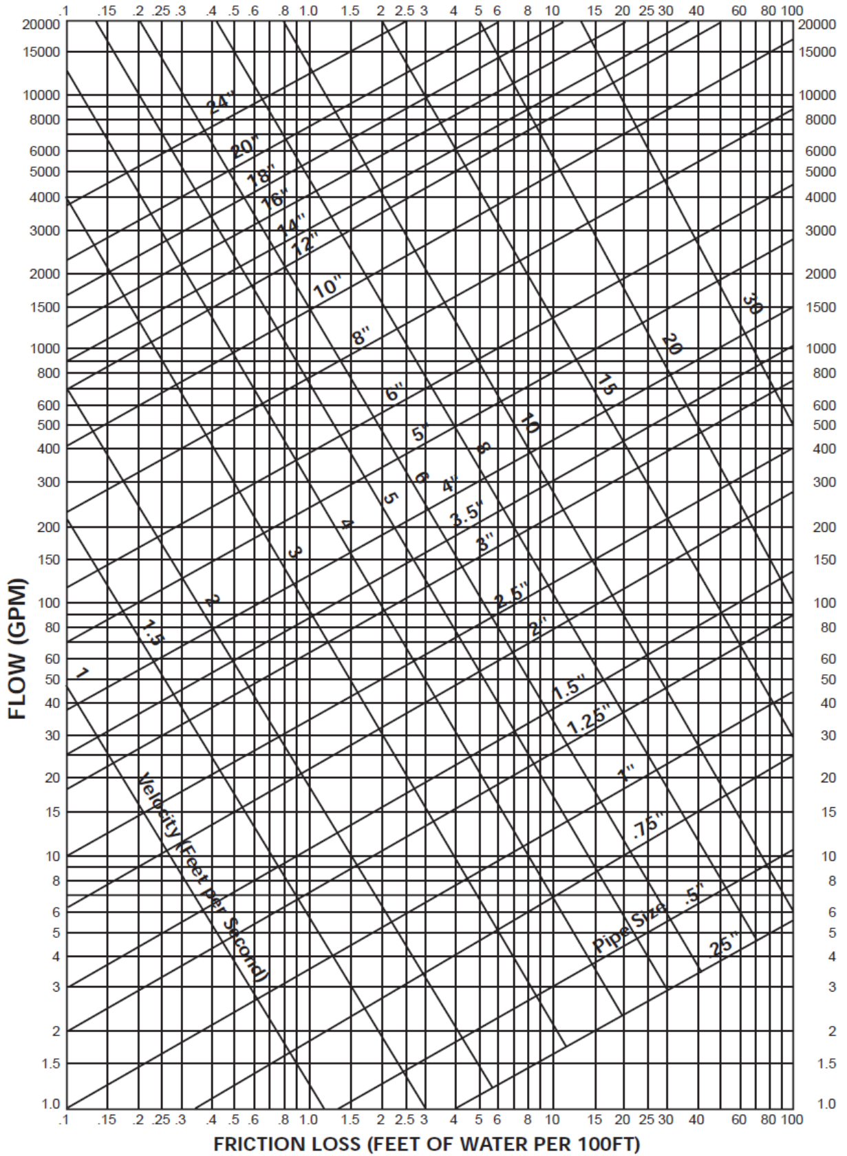
Figure 3-F-1: Friction Loss for closed piping Systems (Water) Schedule 40 Pipe
